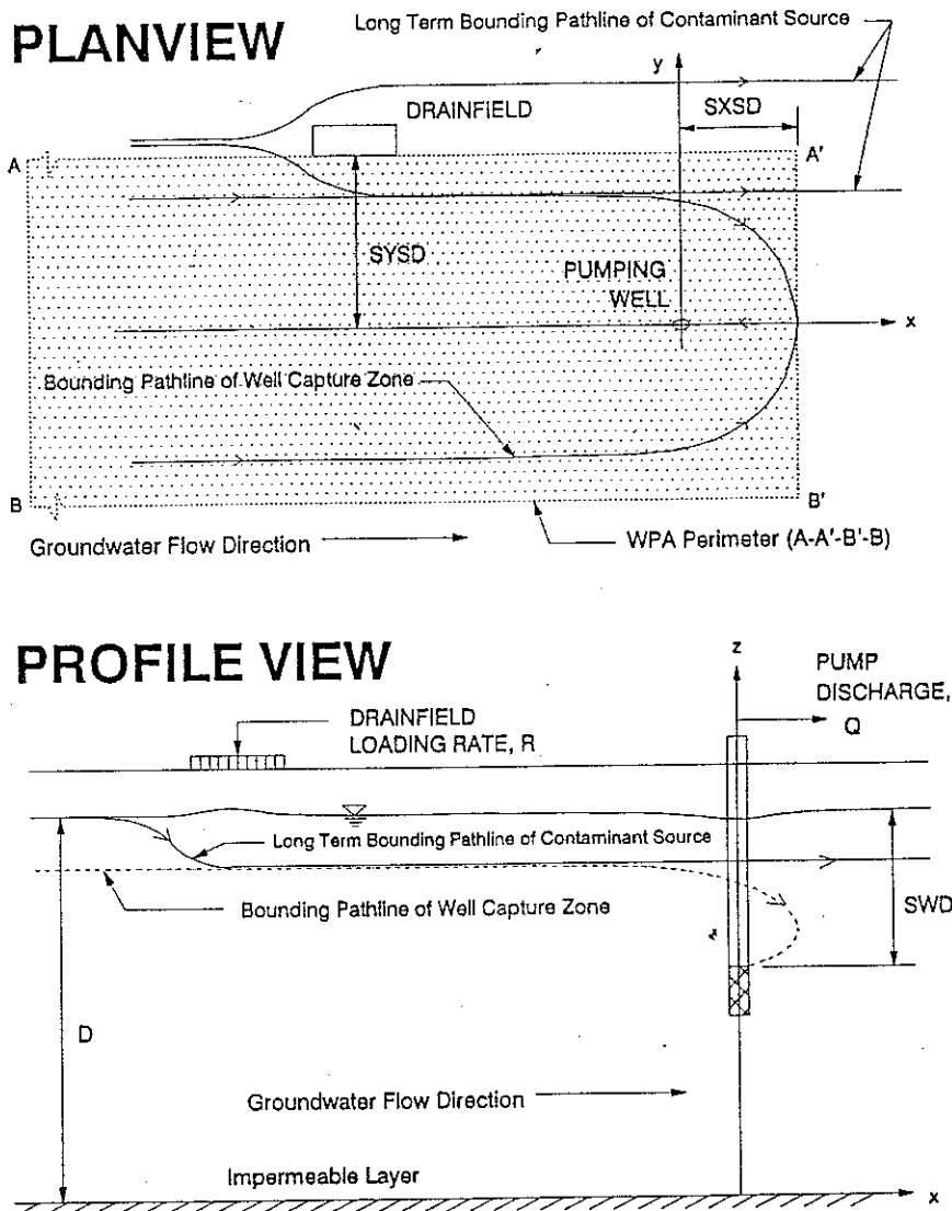
Fig. 1 The Safe X and Y Separation Distances (SXSD, SYSD), Well Protection Area (WPA) (planview, top) and Safe Well Depth (SWD) (profile view, bottom).
