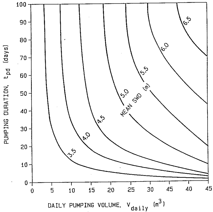
Fig. 2 The Mean SYSD and SWD with Pumping Duration and Daily Pumping Volume.
