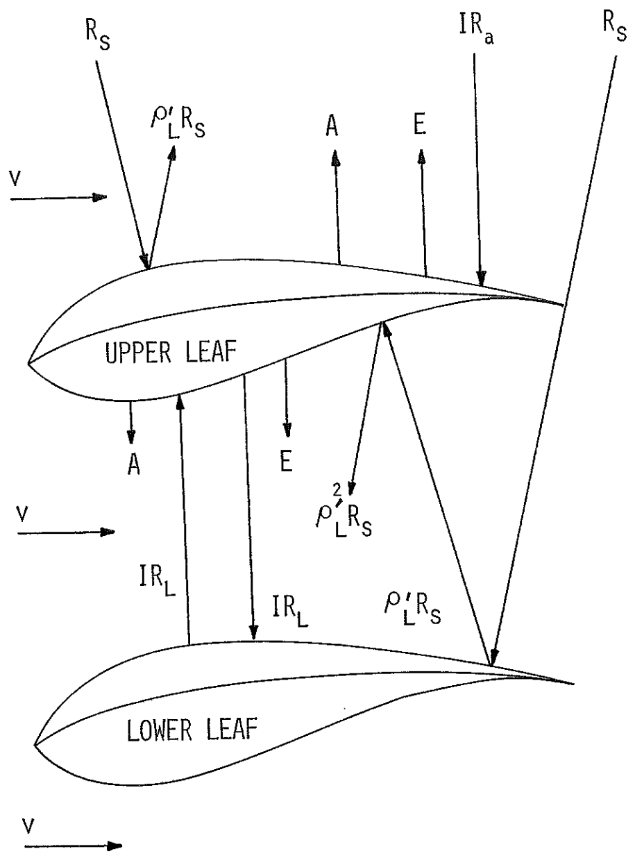
3.1 Leaf energy exchange in field.
