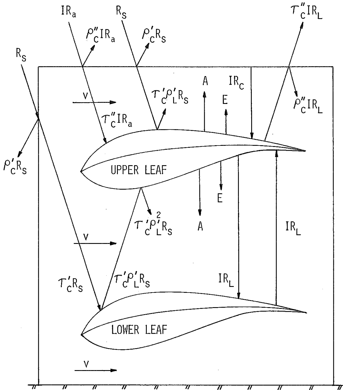
3.2 Energy exchange of leaf enclosed in measurement chamber.
