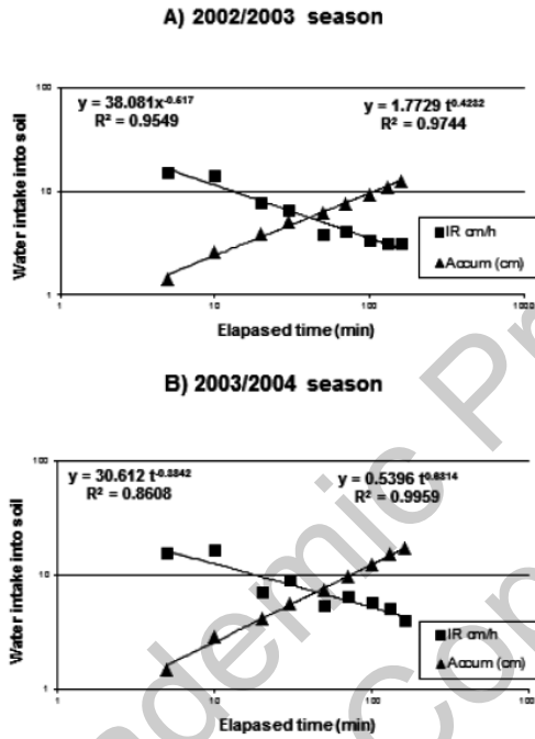
FIGURE 5 Water intake into soil in low-head bubbler irrigation system.
