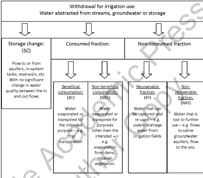
FIGURE 1 ICID water-balance framework for irrigation water management [9].
