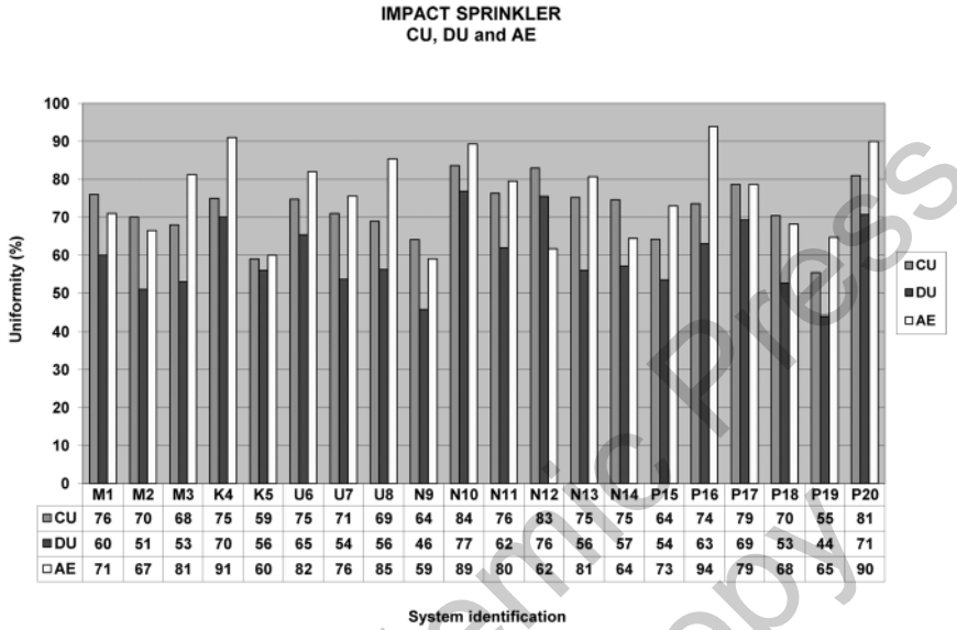
FIGURE 2 Performance of impact sprinkler systems.
