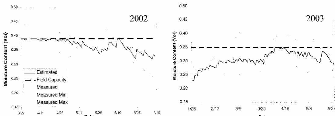
Figure 3. Estimated and measured volumetric soil moisture content between 27 March and 9 July 2002, and 27 January and 12 June 2003.
