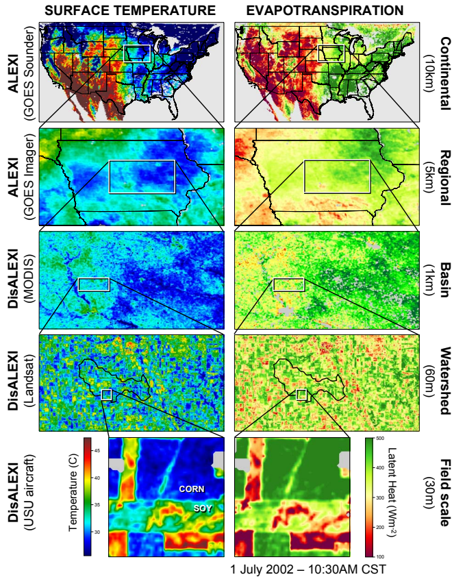
Figure 6 (Left): Multi-scale ET maps for 1 July 2002 produced with ALEXI/DisALEXI using surface temperature data from aircraft (30-m resolution), Landsat (60-m), MODIS (1-km), GOES Imager (5-km) and GOES Sounder (10-km), zooming into the Walnut Creek Watershed near Ames, Iowa, site of the SMEX02 Soil Moisture Experiment. The continental-scale ET map is a 14-day composite of clear-sky model estimates. Application of the DisALEXI model is shown on the bottom left (Anderson et al. 2007c).
